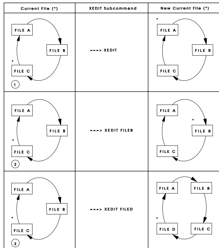
Figure 29. Editing Files in the Ring
