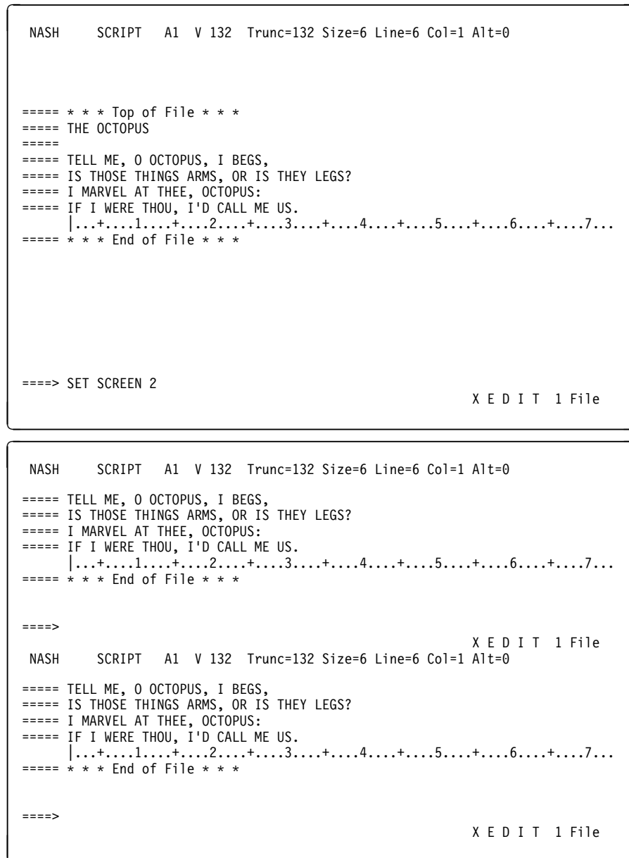
Figure 30. Multiple Horizontal Views of the Same File
