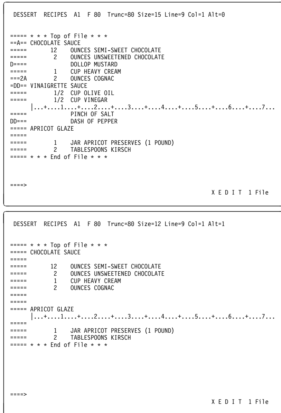
Figure 7. Prefix Subcommands A and D — Before and After
